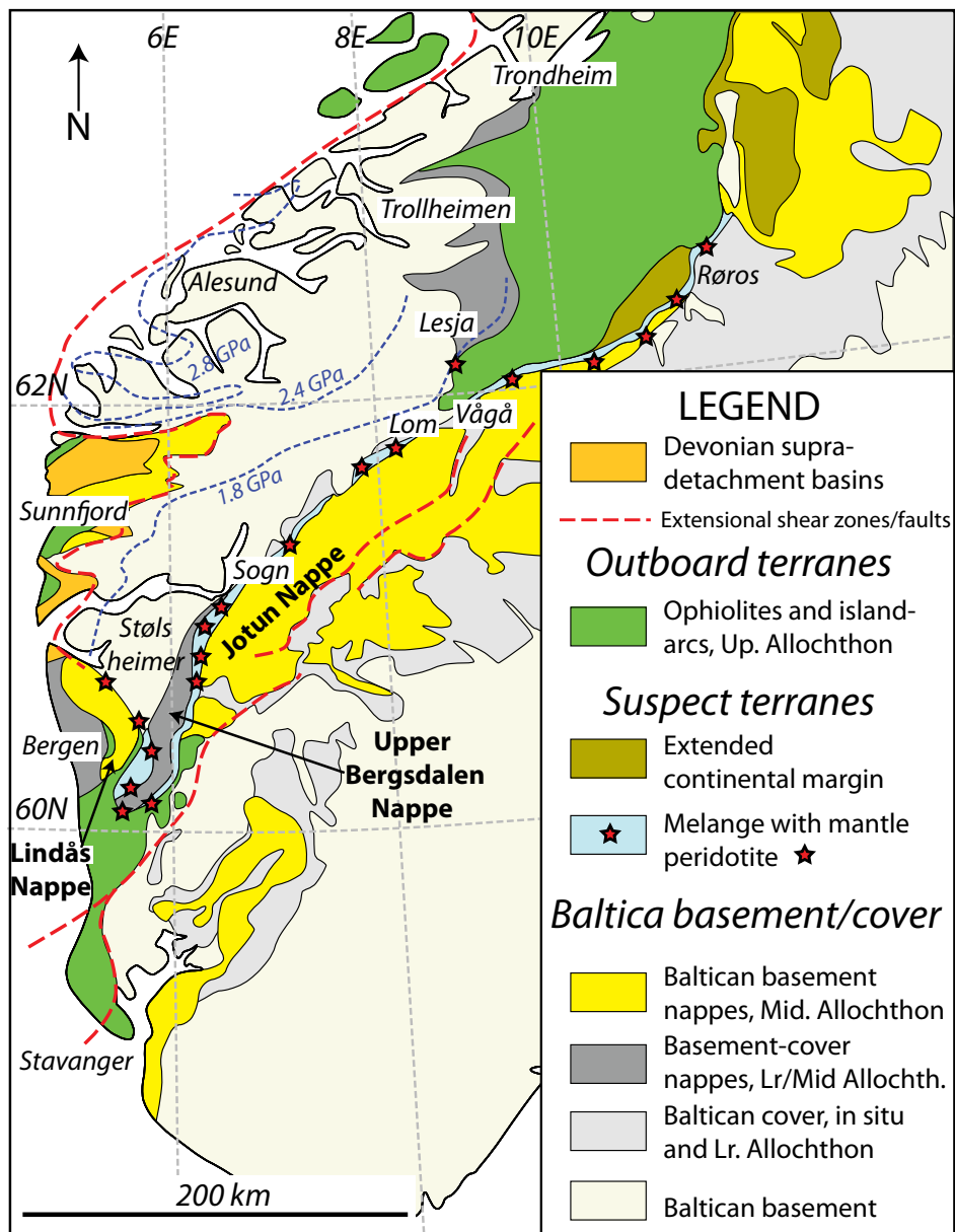
Figure 9. Tectonostratigraphic map of the South Norwegian Caledonides (from Andersen et al. 2012), highlighting the regional distribution of the hyper-extended mélange assemblages structurally below the large crystalline nappes (such as the Lindås, Upper Bergsdalen and Jotun Nappes) of the Middle Allochthon.
