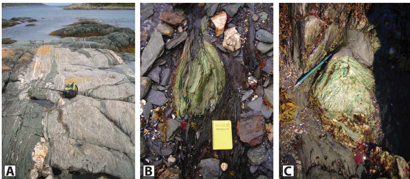
Figure 6. (A) Isoclinal fold closures within interlayered mafic schist and psammitic wackes in the Birchy Complex, western Newfoundland. Small podiform serpentinite clasts enclosed by B) graphitic pelite, and C) mafic schist, in the Birchy Complex.
