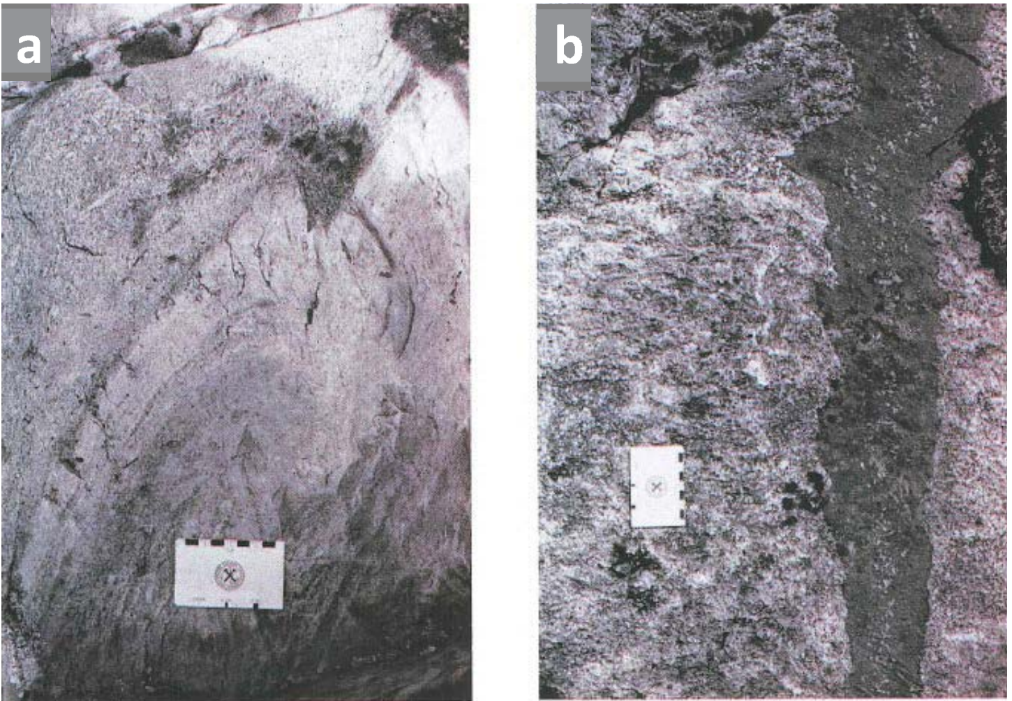
Figure 27. (a) Rhyolite lobe from Neoarchean Confederation assemblage in the Red Lake greenstone belt. (b) Rhyolite tuff from Neoarchean Confederation assemblage; the tuff breccia is cut by a plagioclase-phyrlic andesite dyke. Centimetre scales are shown. From Sanborn-Barrie et al. (2000).
