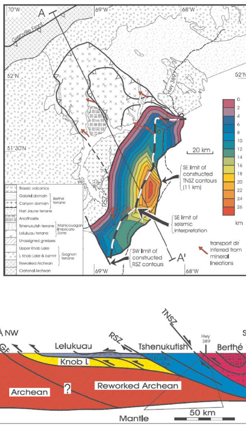
Figure 16. (a) Isopach map for the Tshenukutish terrane. Heavy dashed line is the southeastern limit of structure contours for which their position is constrained by observed reflectors. Red arrows show inferred transport directions for rocks within Tshenukutish terrane based on the predominant trends of mineral lineations. AA' is location of section below. (b) Vertical cross-section along line AA' (Figs. 15a, 16a). Depths of boundaries within the triangular field beneath the surface trace of Highway 389 are constrained by structure-contour maps derived from interpretation of Line 55. Outside that region, subsurface structure is based on extrapolation parallel to the regional tectonic trend of the Grenville orogen. Colour and ornament same as Figure 15a. From Hynes et al. (2000).
