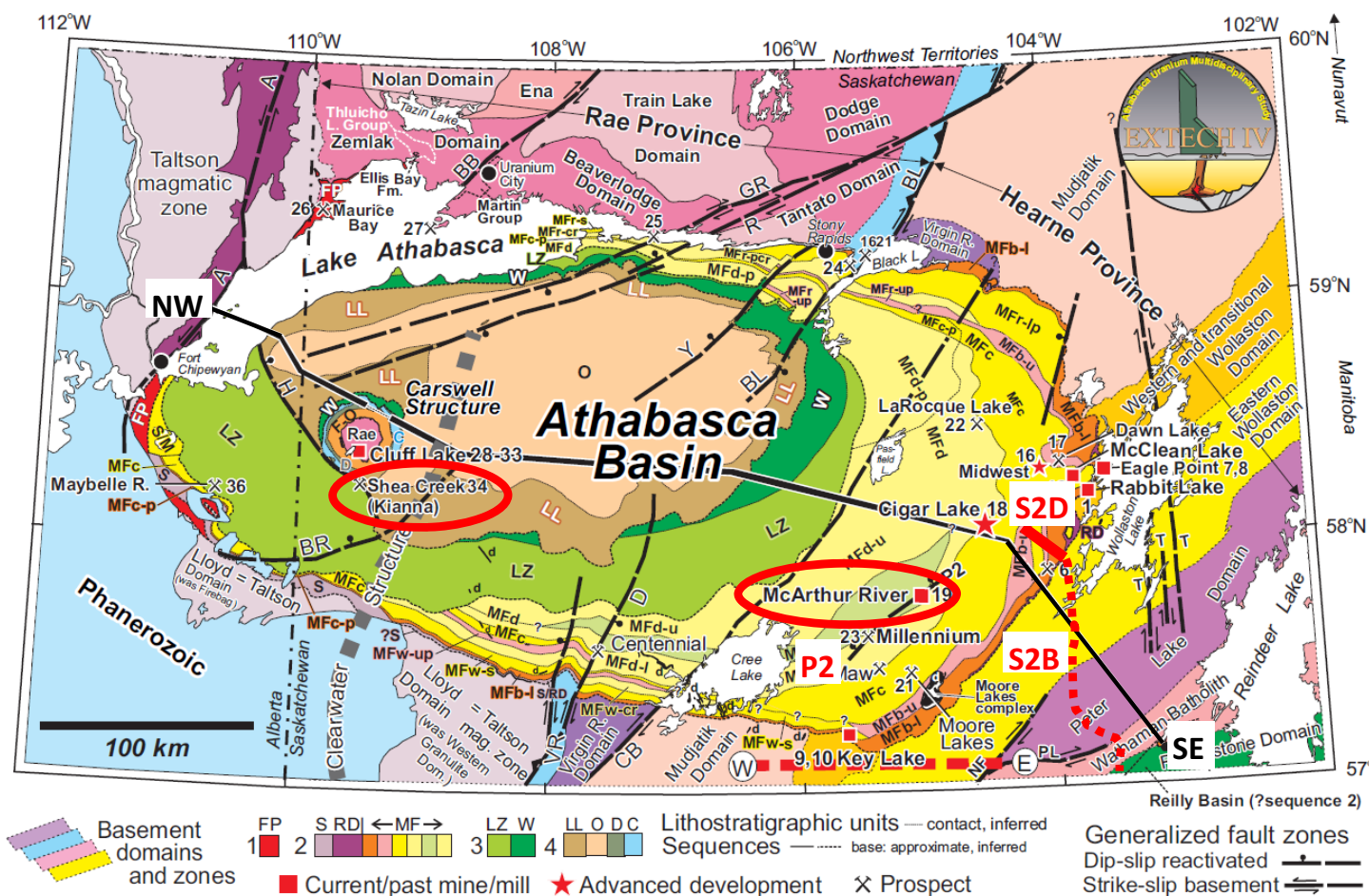
Figure 22. Geological setting and unconformity-associated uranium occurrences (numbered) of the Athabasca Basin region of northern Saskatchewan and Alberta. Symbols and fonts are slightly larger for more significant occurrences. Abbreviations for geological sequences, formations and members shown in the legend: Sequence 1: FP, Fair Point; Sequence 2: S, Smart; RD, Read; MF, Manitou Falls (members identified with different colours and letters on map); Sequence 3: LZ, Lazenby Lake; W, Wolverine Point; Sequence 4: LL, Locker Lake; O, Otherside (also called William River); D, Douglas; C, Carswell. P2 identifies the P2 reactivated thrust fault. The black line NW–SE is the location of the cross-section in Figure 23. Seismic lines S2D and S2B are located. Red ellipses highlight the two deposit areas discussed in this section. For further information, see Jefferson et al. (2007) from which the map was extracted.
