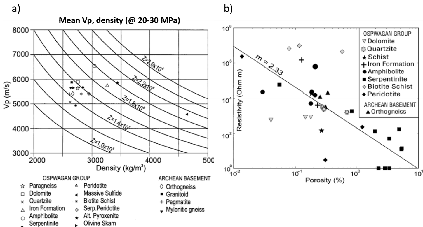
Figure 13. a) Mean P -wave velocities ( V_p ) and densities for a suite of rocks from the Thompson area. The solid curves indicate lines of constant acoustic impedance (product of V_p and density with units of \text{kg/m}^2 \text{s} ). The V_p and density values for the massive sulphide are for a pyrrhotite-rich sample from Sudbury because no measurements were available for such sulphide rocks from the Thompson area. From White et al. (2000). b) The log of resistivity versus the log of porosity for a suite of samples provided by Inco Ltd., Exploration. These rock property results were used to facilitate the interpretation of conductivity in terms of ionic transport (i.e. via fluids) versus electronic conductors (i.e. metals and semiconductors). From White et al. (2000).
