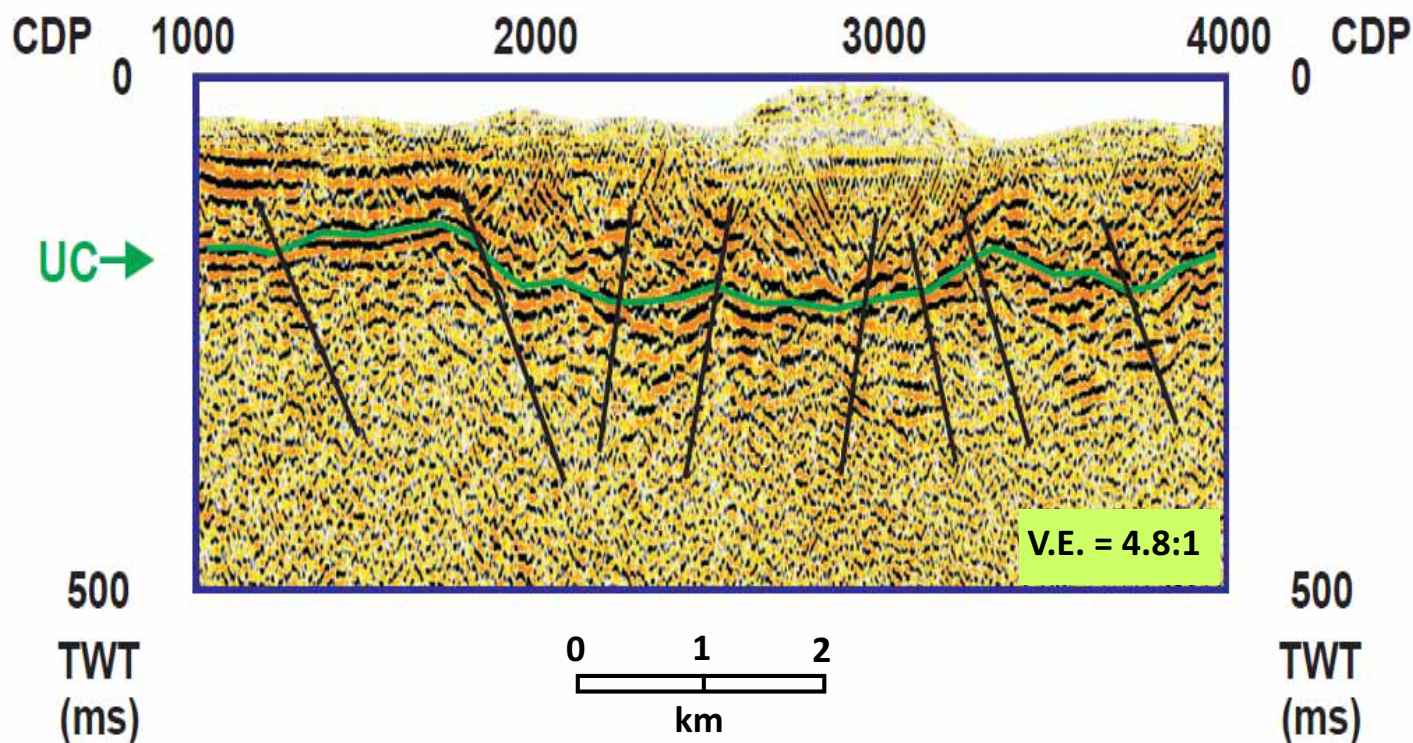
Figure 26. Enlarged example of the seismic image of the unconformity (UC) and associated fault system that extends from the basement into the overlying sandstone as observed on Lithoprobe's high resolution seismic profile S2D (location in Fig. 22). Figure from Hajnal et al. (2010).
