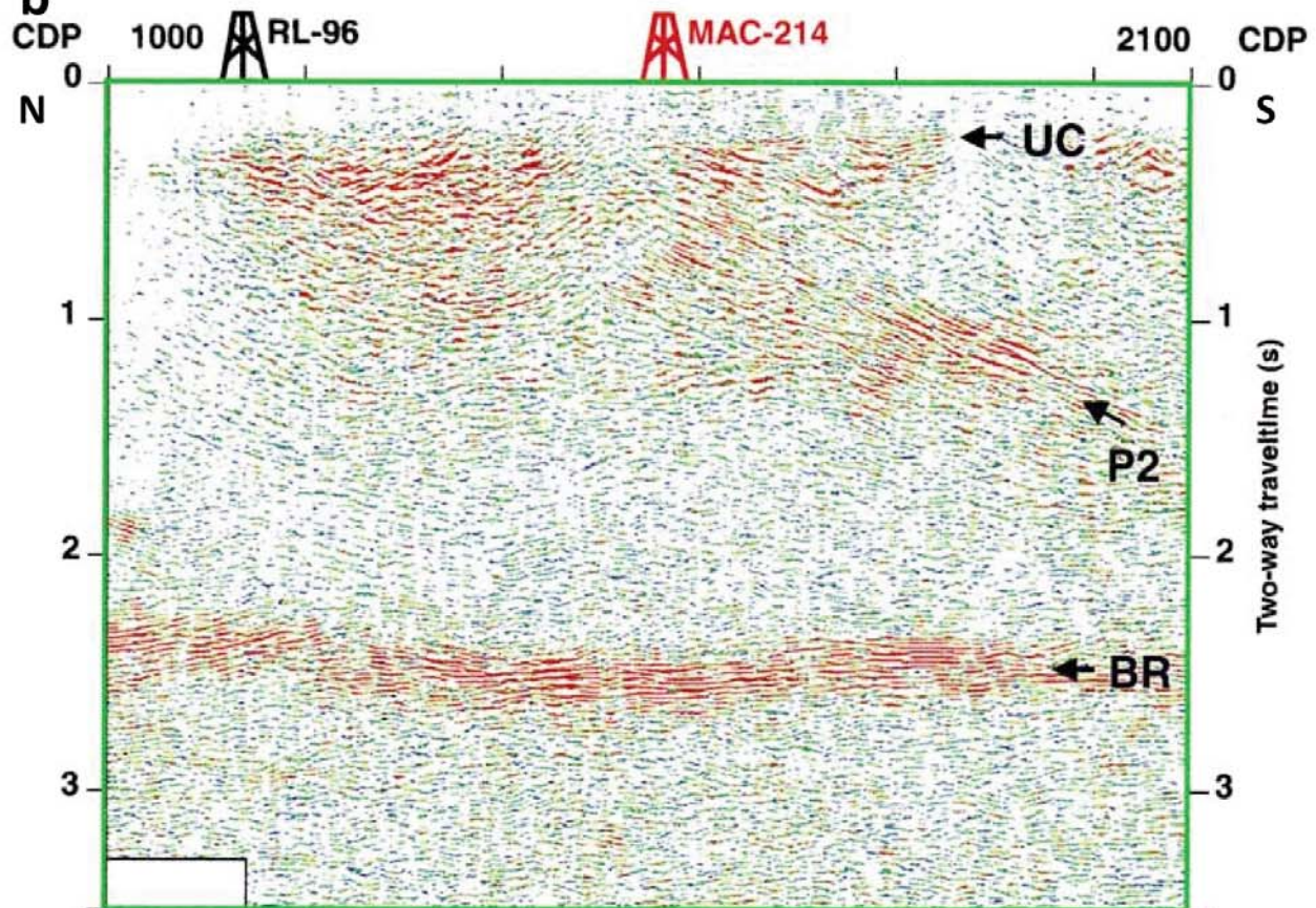
Figure 29. a) Total field magnetic map of the McArthur River study area with lithotectonic domains shown. Seismic lines are identified. Numbers are common-depth-point (CDP) locations. The white rectangle outlines the location of the low-fold 3-D acquisition program. b) Enlarged portion of line B-B', CDPs 1000 to 2100 (~12 km). Drillhole locations are marked. UC, unconformity; P2, the P2 reverse fault zone; BR, bright reflector. From Hajnal et al. (2007).
