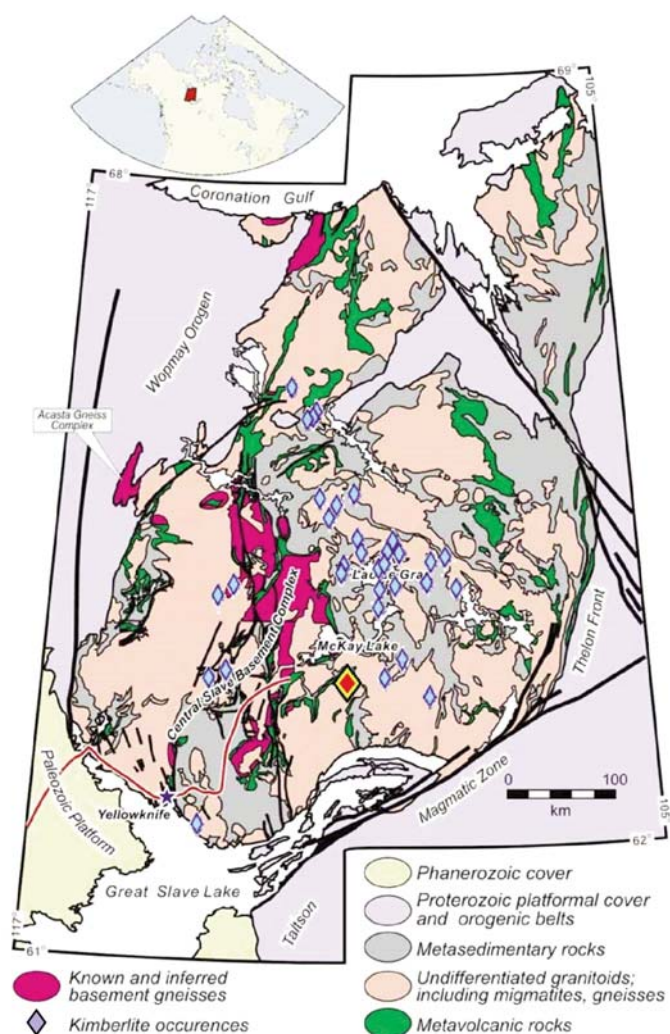
Figure 31. Geologic map of the Slave Province; inset shows location in North America. The Archean cratonic core is bounded by fault zones (bold lines), orogenic belts, and platform cover. Red and yellow diamond, Snap Lake study location; blue diamonds, known kimberlite pipes, dykes, and sills. Modified from Bleeker and Davis (1999).
