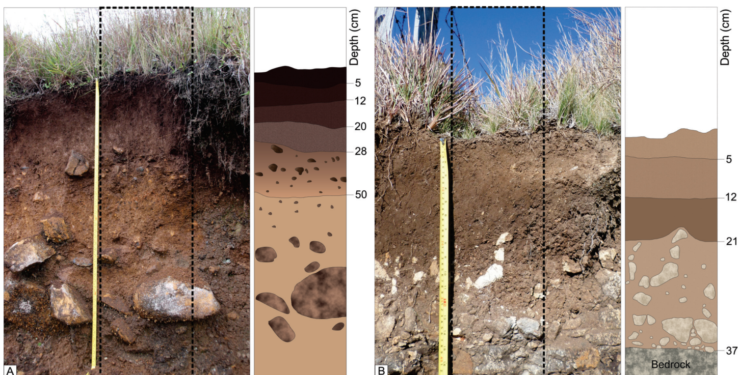
Figure 9. Detailed soil profiles: (A) Inceptisols (sample SJE-004) and (B) Entisols (sample SJE-006). Schematic drawings summarize soil horizons and depth. São Joaquim, State of Santa Catarina.
