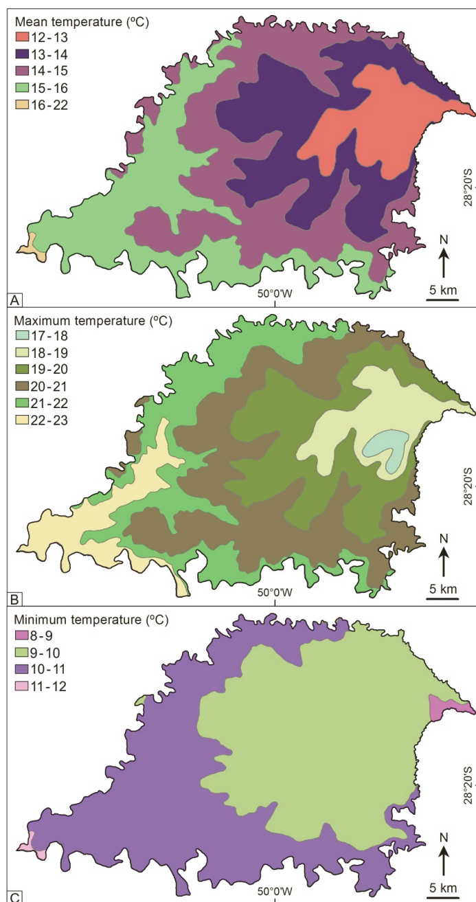
Figure 4. Meteorological maps of the municipality of São Joaquim: (A) annual mean temperature, (B) annual maximum temperature and (C) annual minimum temperature. Modified from Pandolfo et al. (2002).
