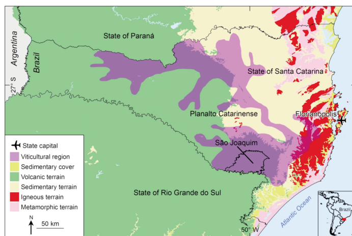
Figure 1. Location map of the Planalto Catarinense viticultural region and the municipality of São Joaquim, State of Santa Catarina, Brazil. Geological data from CPRM (2015).
