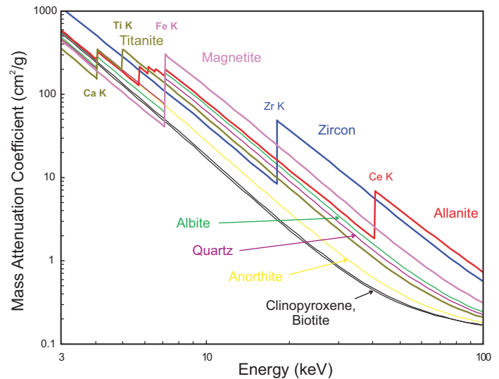
Figure 5. Energy dependence of X-ray absorption (after Gualda et al. 2010). Although absorption increases with decreasing X-ray energy, there are discontinuities at the characteristic energy for each element. Subtraction of images obtained at energies above and below the discontinuity can give an image of that element only.
