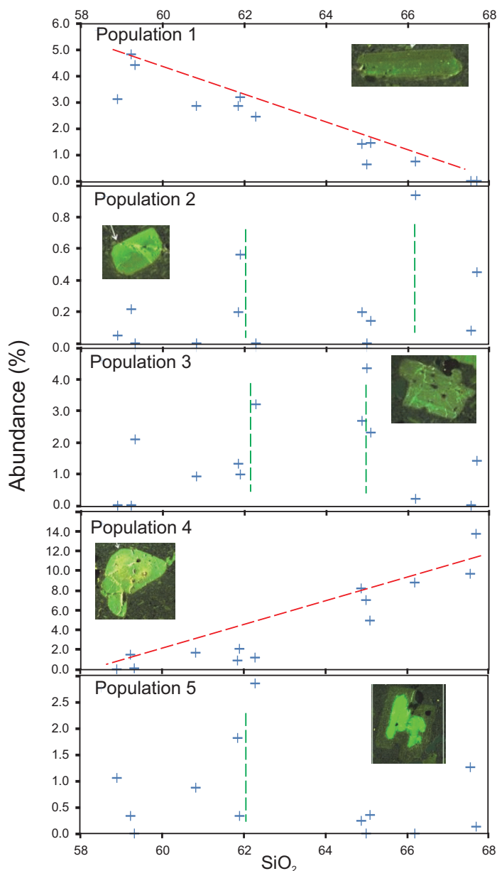
Figure 9. Abundance of five different crystal populations versus overall \text{SiO}_2 content in dacite lavas from Quizapu volcano, Chile (Voos 2013). Linear variations suggest that two populations are associated with the andesite and dacite end-members. The other three populations represent specific batches of magma mixed at depth. Such complex mixing behaviour necessitates an elaborate magmatic plumbing system beneath the volcano.
