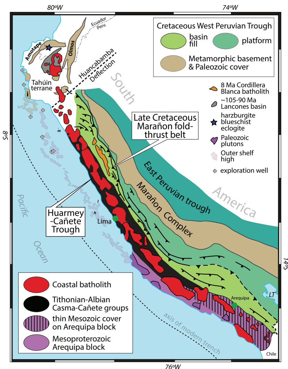
Figure 1. Geological sketch map of western Peru illustrating the general relations between Tithonian–Albian rocks of the Casma Group deposited in Huarmey basin, the Coastal batholith, and the West Peruvian Trough. Location of the Early Cretaceous subduction complex (harzburgite–blueschist–eclogite), which predated the events in this paper as the rocks there were exhumed during the Early Cretaceous, is from Feininger (1980). i –Illascas massif; m –Isla Macabi; b –Isla de las Hormigas de Afuera; L –Isla Lobera; LT –Lake Titicaca.
