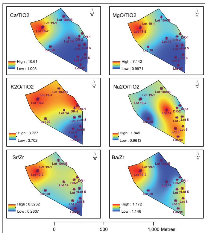
Figure 8. Map showing the spatial distribution and degree of chemical weathering in the Wollersheim Winery vineyards (see Figs. 2, 4), using ratios of selected mobile to immobile elements. More extensive chemical weathering is associated with vineyards in the north, east, and south.
