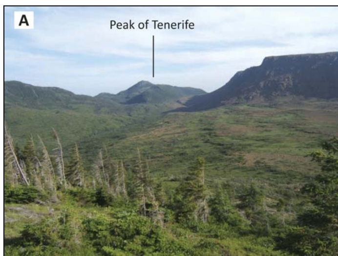
Figure 22. Stop 2.5 located on the metamorphic aureole of the Tablelands Ophiolite. (A) The contrast between the eastern edge of the ophiolite (at right) and the forested hills of the metamorphic aureole, including the Peak of Tenerife. (B) Foliated and lineated fine-grained amphibolitic rock of the aureole, likely derived from mélangé including mafic volcanic material.
