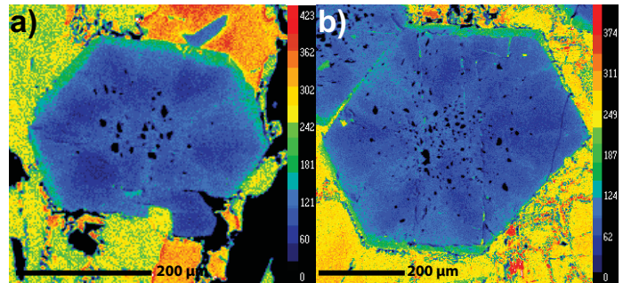
Figure 12. Mg X-ray maps in sector-zoned garnet from the St. Cyr klippe. Eclogite samples (a) 10-143 and (b) 10-06. Warm colors represent higher elemental concentrations.
