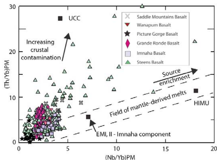
Figure 18. Diagram showing variation in (\text{Nb}/\text{Yb})_{\text{PM}} and (\text{Th}/\text{Yb})_{\text{PM}} . The ratios are normalized to primitive mantle values (PM) of McDonough and Sun (1995) following Jowitt and Ernst (2013) and Jowitt et al. (2014). N-MORB is from Hofmann (1988); Upper Continental Crust (UCC) composition is from Taylor and McLennan (1985) and Enriched Mantle (EMI, EMII – the Imnaha component of Hooper and Hawkesworth 1993) and HIMU values concentrations from Condie (2001). This diagram assesses the probability of the Columbia River Basalt Group magmas assimilating significant amounts of crustal material prior to emplacement. Note that the Grande Ronde, Upper Steens, Wanapum and Saddle Mountains Basalts show evidence of crustal contamination. Picture Gorge, Imnaha, and Lower Steens Basalts indicate little crustal contamination as has been shown by Hooper and Hawkesworth (1993), and Camp and Hanan (2008).
