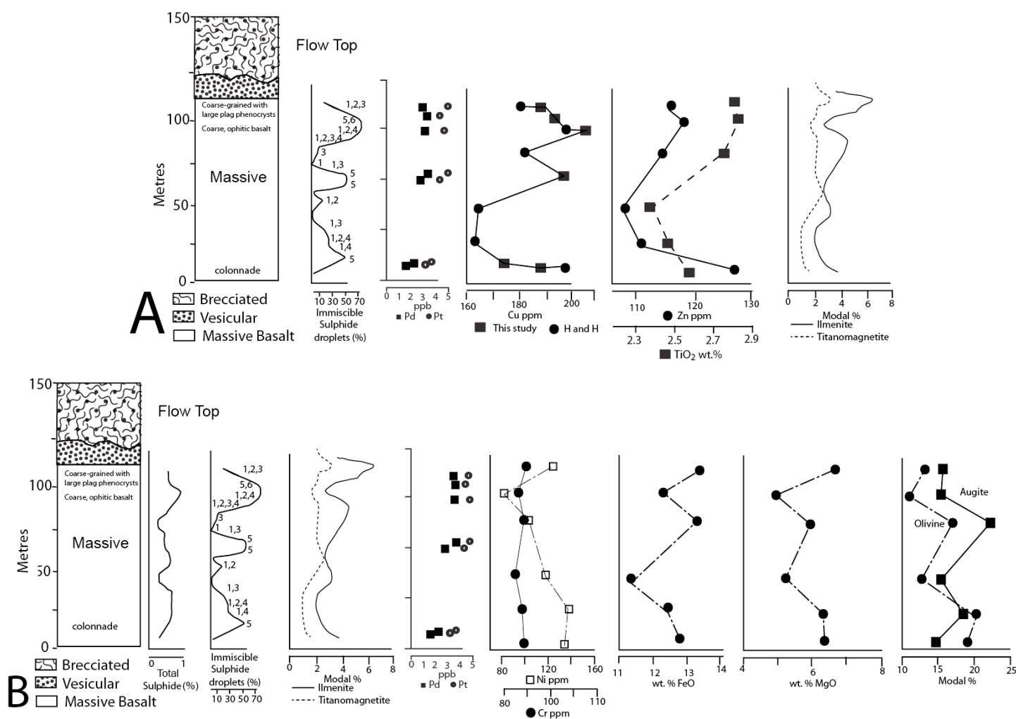
Figure 10. Compositional and mineralogical concentrations in the Rock Creek flow, Imnaha Basalt. A) Pt, Pd, Cu, Zn, Ilmenite, titanomagnetite, sulphides; B) Pt and Pd, Ni, Cr, MgO, \text{Fe}_{\text{Total}} as FeO, and modal olivine and pyroxene, ilmenite, titanomagnetite and sulphides. Pt and Pd from this study, immiscible sulphide, total sulphides, and Ilmenite and titanomagnetite abundances from Korzendorfer (1979) and Ni, Cr, MgO, \text{Fe}_{\text{Total}} , and modal olivine and pyroxene from Holden and Hooper (1976) with samples reanalyzed by this study. For Immiscible Sulphide Droplets, 1 = mainly pyrrhotite with some chalcopyrite; 2 = equal amounts of pyrrhotite and chalcopyrite; 3 = mainly chalcopyrite; 4 = chalcopyrite and exsolved (?) cubanite; 5 = mainly goethite with chalcopyrite and small amount of unknown mineral; 6 = mainly bornite with chalcopyrite and minor titanomagnetite from Korzendorfer (1979).
