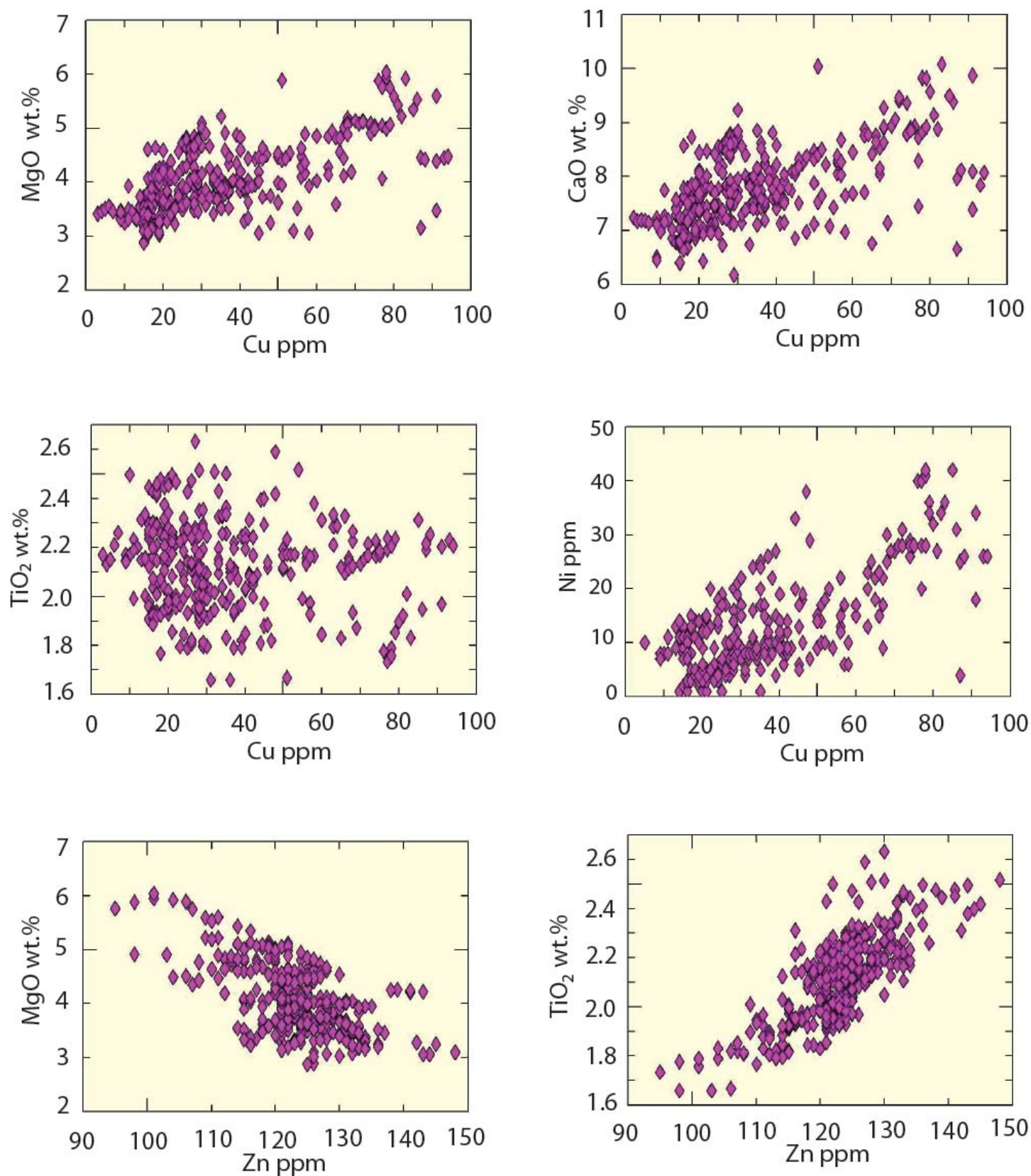
Figure 14. Variation diagrams for Cu vs. MgO, TiO 2 , CaO and Ni, and Zn vs. MgO and TiO 2 for the Grande Ronde Basalt. Data from Reidel and Tolan (1992, 2013), Schuster (1993), Hooper and Hawkesworth (1993), Hooper (2000), Reidel (2005) and S. Reidel unpublished data.
