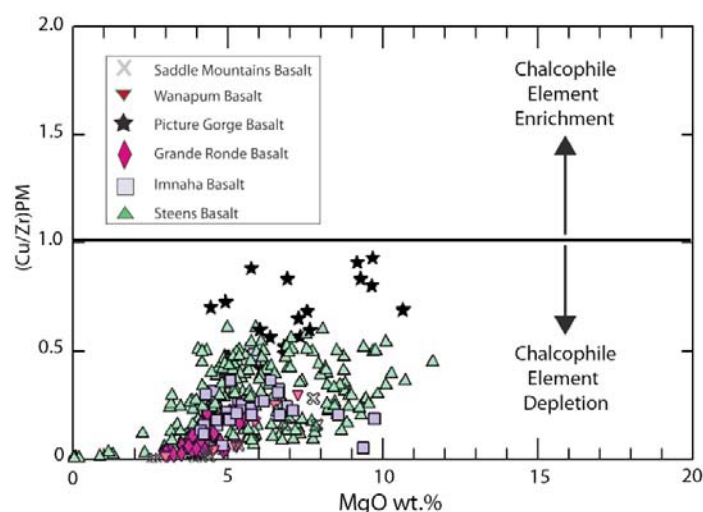
Figure 17. Diagram showing (\text{Cu}/\text{Zr})_{\text{PM}} and MgO. The ratios are normalized to primitive mantle values (PM) of McDonough and Sun (1995) and Jowitt et al. (2014). This figure shows the abundance of chalcophile elements in the CRBG. The Cu/Zr(PM) reflects the sulphide budget of the magma and suggests that all formations are greatly depleted in Cu with the Steens Basalt and Picture Gorge Basalt being the least depleted. The most depleted are the Grande Ronde Basalt, Wanapum Basalt and Saddle Mountains Basalt, the last formations to be emplaced.
