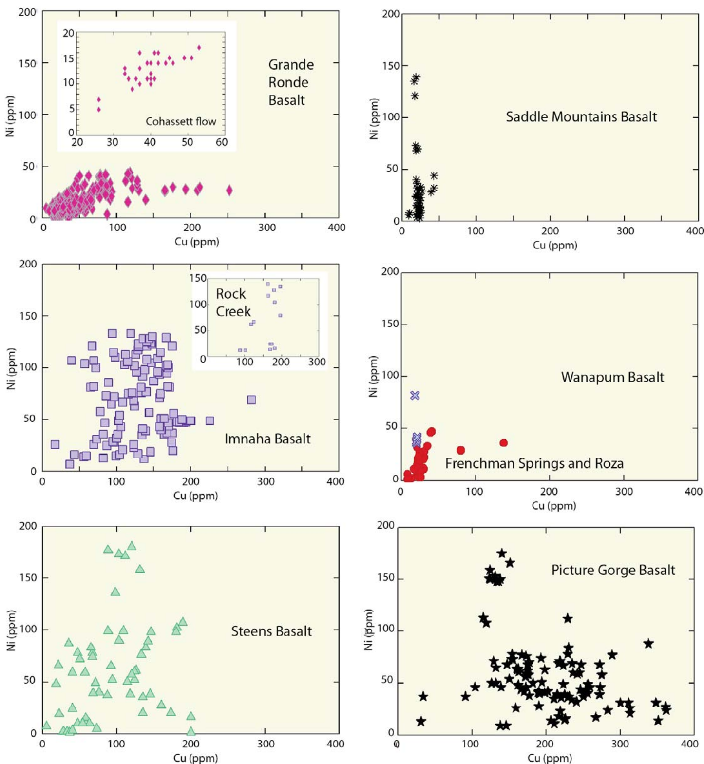
Figure 8. Variation diagram for Cu and Ni in the Columbia River Basalt Group. Data from Bailey (1989), Schuster (1993), Hooper (2000), Camp et al. (2003, 2013), Wolff et al. (2008 Appendix), Reidel and Tolan (2013), and S. Reidel unpublished data. For Wanapum Basalt, circle is Frenchman Springs Member and 'x' is Lolo flow, Priest Rapids Member (see Fig. 2).
