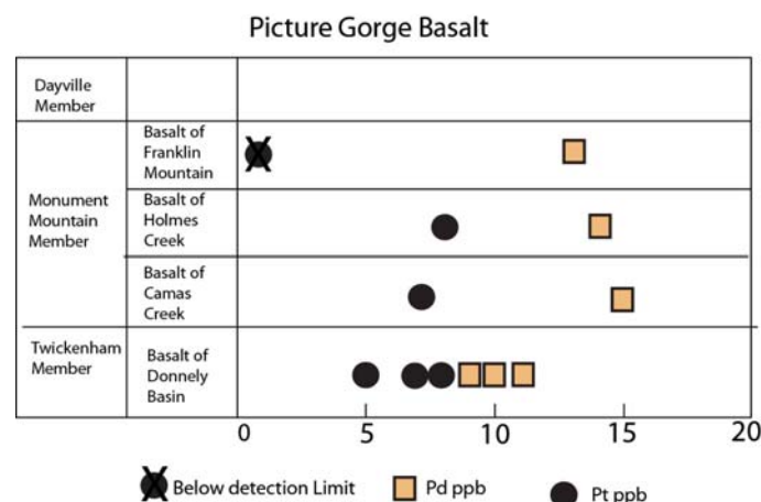
Figure 15. Pt and Pd abundance in Picture Gorge Basalt. Stratigraphic nomenclature based on Bailey (1989). Data from this study (Table 2).
