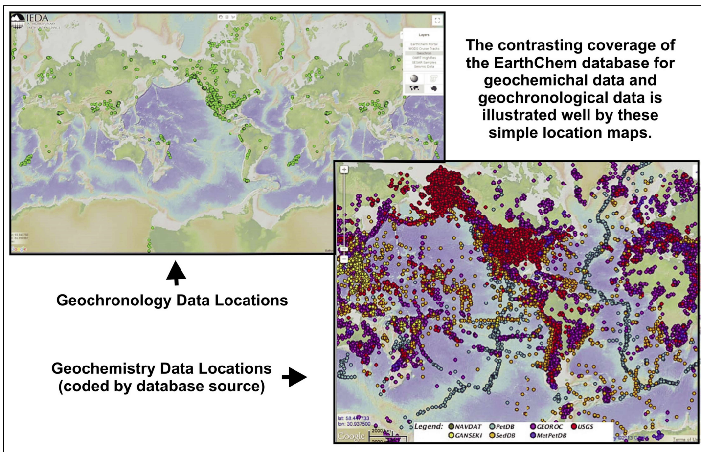
Figure 2. Maps produced from the EarthChem database showing the geographical restrictions of geochronological data compared to lithogeochemical data. IEDA = Interdisciplinary Earth Data Alliance. Figure sources: http://earthchem.org/portal (geochemistry sample image); http://app.iedadata.org/databrowser/ (geochronology image).
