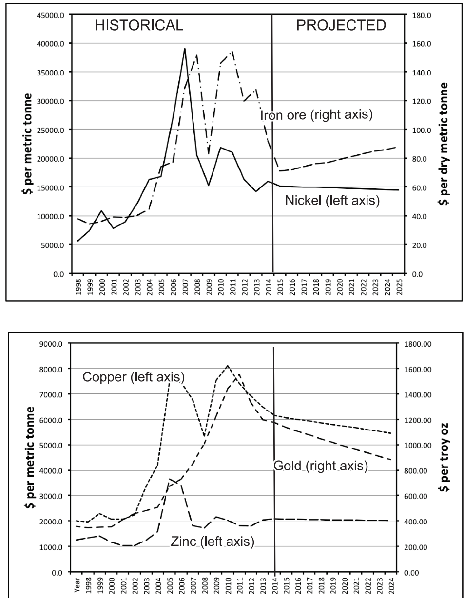
Figure 1. The history of the commodity boom and subsequent decline as revealed by selected metal prices in constant US dollars. Prices to the right of the vertical line are projected. Source World Bank (2015).
