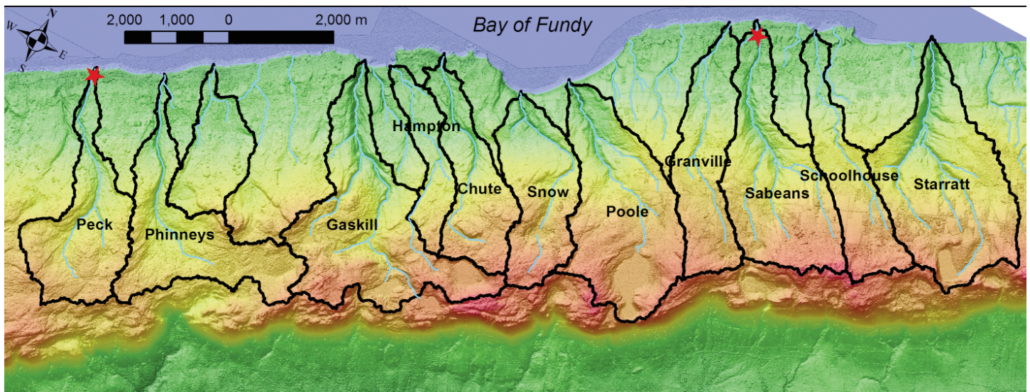
Figure 2. Labeled catchment basins (black lines) calculated from the lidar DEM for North Mountain. The blue lines denote the main truck streams within the basins. The two red stars denote the location of stream discharge and water chemistry sensors in Peck and Sabeans basins.
