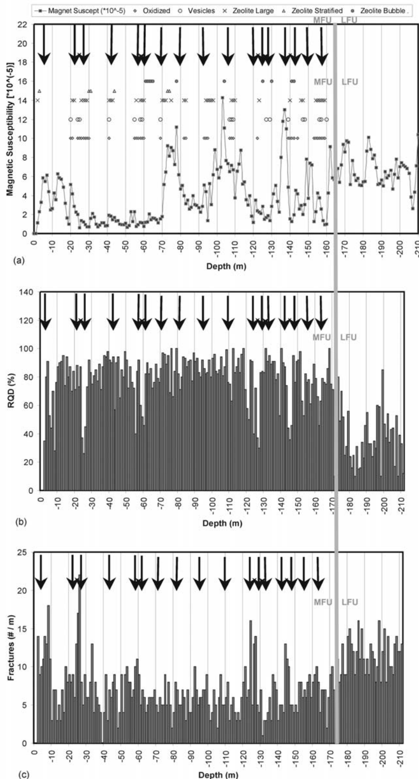
Figure 7. Plots of drill core logs of drill hole GAV77-3 for the North Mountain Basalt. The heavy grey vertical line marks the contact between the Middle Flow Unit (MFU) and Lower Flow Unit (LFU). (a) Magnetic susceptibility and the distribution of oxidized basalt, vesicles and amygdulites interpreted to represent flow tops. The arrows denote individual flows within the MFU. The boundary between the MFU and LFU occurs at depth 162 m. (b) Rock Quality Designator (RQD) %, which is the cumulative percentage of the number of pieces of core that are larger than 10 cm over a distance of 1 m. (c) Number of fractures per metre length of core.
