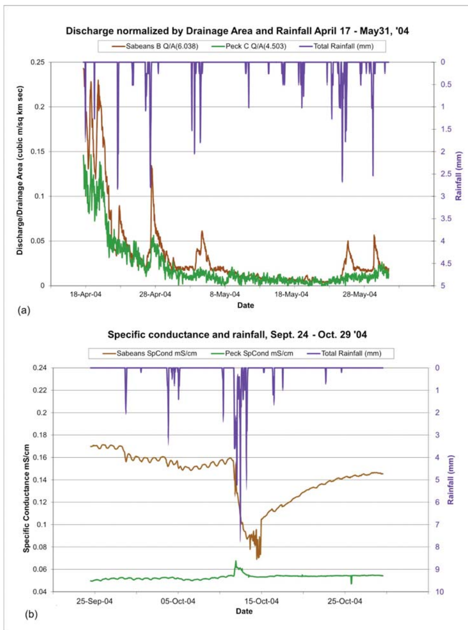
Figure 8. Hydrographs and water chemistry plots of representative basins from the till blanket (TB) area (Sabeans Brook catchment dark grey) and the scoured bedrock till veneer (TV) area (Peck Brook catchment light grey). (a) Hydrographs of Sabeans Brook and Peck Brook basins, discharge \text{m}^3/\text{s} normalized by basin drainage area ( \text{km}^2 ) for the period of April 17 to May 31, 2004. Rainfall (mm) is plotted in reverse order on the right y-axis. (b) Specific conductance (microseimens per centimetre) and rainfall for Sabeans Brook and Peck Brook for the period of September 24 to October 28, 2004.
