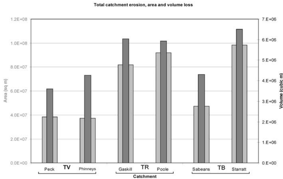
Figure 6. Graph of area and volume of erosion for each basin along the North Mountain Basalt. The basins have been grouped based on the degree of glacial till cover: TV – thin till veneer, TR – transition zone with till in the headwaters, and TB – thick till blanket. The thicker light grey bars represent total area (left axis) of material removed per basin and the thinner dark grey bars represent the total volume (right axis) of material removed per basin.
