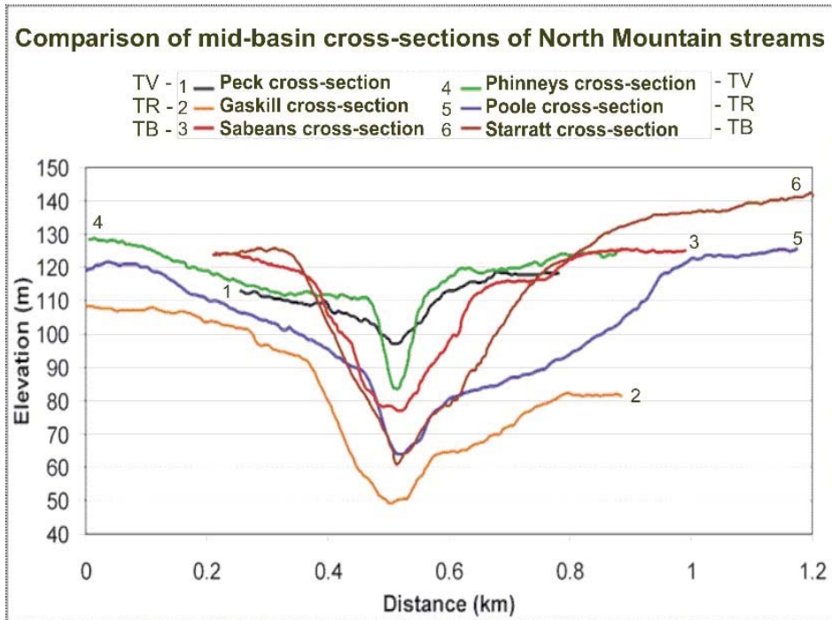
Figure 3. Mid-basin cross-sections of catchments from west to east on North Mountain with variable amounts of till cover. Cross-sections for the approximate midpoint of each basin are labeled: 1 – Peck, 2 – Gaskill, 3– Sabeans, 4 – Phinneys, 5 – Poole, and 6 – Starratt.
