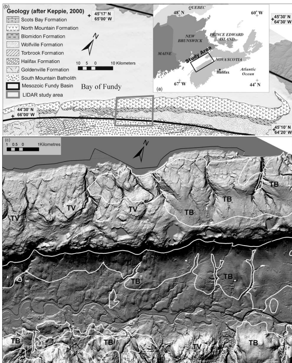
Figure 1. (a) Upper right study area location map (black rectangle). (b) Bedrock geology map (after Keppie 2000) of the Fundy Basin (heavy black rectangle) with lidar DEM location (heavy grey line). (c) Lidar DEM shaded relief model, azimuth angle 315, elevation angle 45; 5 times vertical exaggeration with the distribution of thick till blanket (TB) and thin till veneer (TV) (after Stea and Kennedy 1989).
