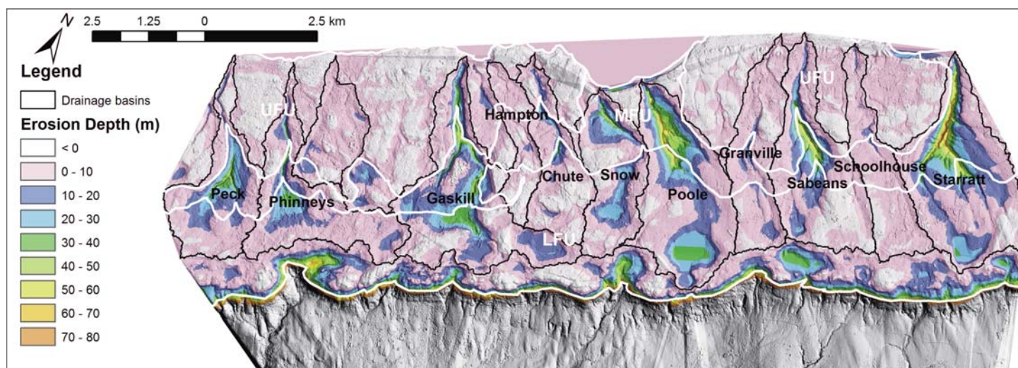
Figure 5. North Mountain drainage basin boundaries (black lines and labels) and erosion depth map with basalt flow unit boundaries (white lines and labels: Lower Flow Unit – LFU, Middle Flow Unit – MFU, Upper Flow Unit – UFU). The western basins have maximum incision depths of approximately 40 m and the central and eastern basins have maximum incision depths approaching 80 m.
